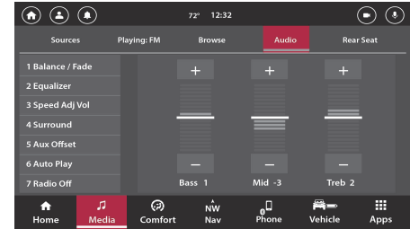
Audio Settings
