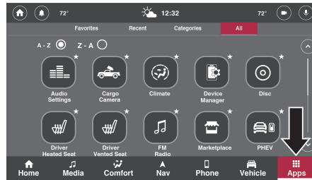
Apps Mode
