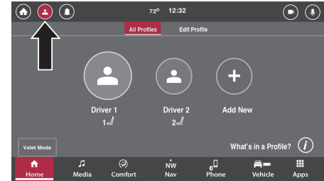
Profile Menu
