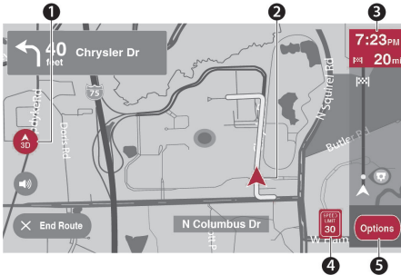
Guidance View
