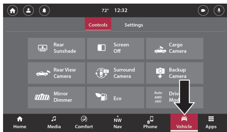
Vehicle Mode
