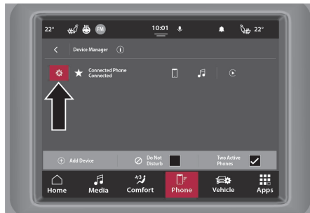
Device Settings
