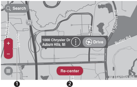
Map View
