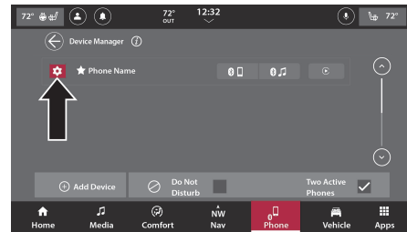
Device Settings
