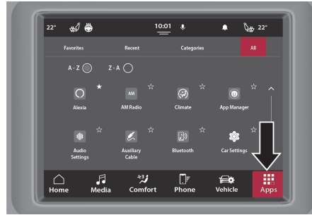
Apps Mode
